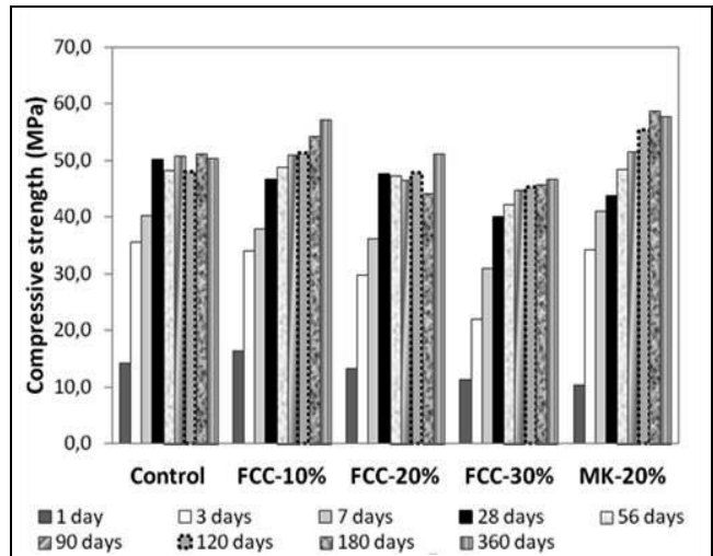
Figure 2. Evolution of compressive strength.
